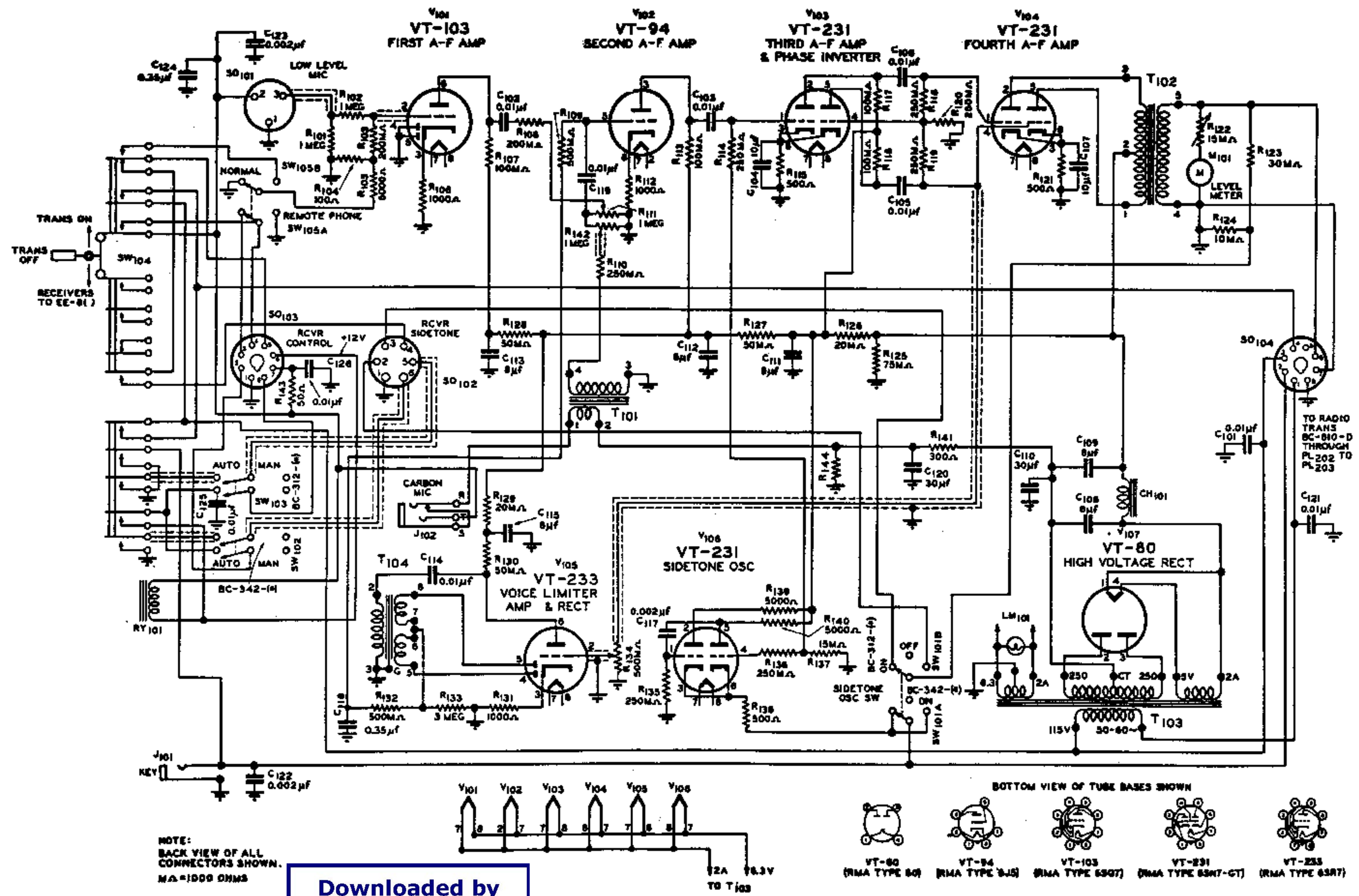
Fig. 3.—Schematic BC-614-D.
