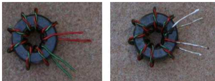
Illustration 19: T-3 Winding Detail (N7VE Photo)
