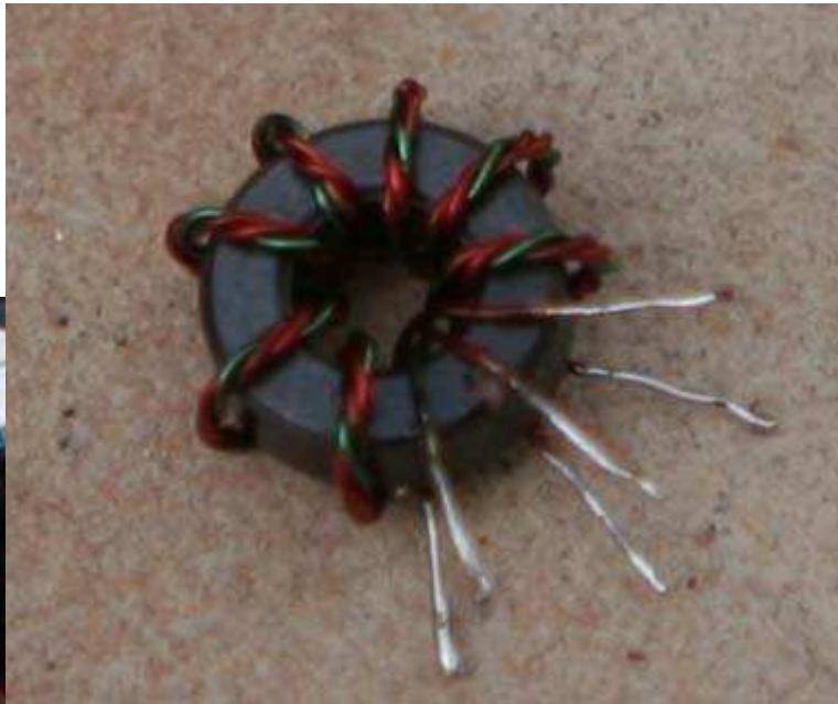
Illustration 20: T-2 Winding Detail (N7VE Photo)
