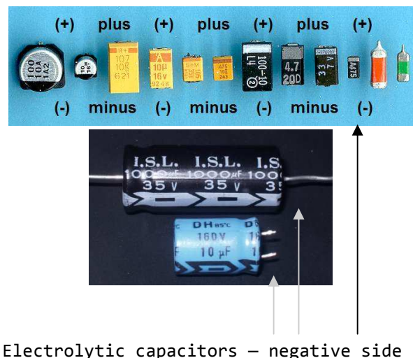
Detail 1. Identifying polarity of diodes, transistors, ICs and polarized capacitors.
