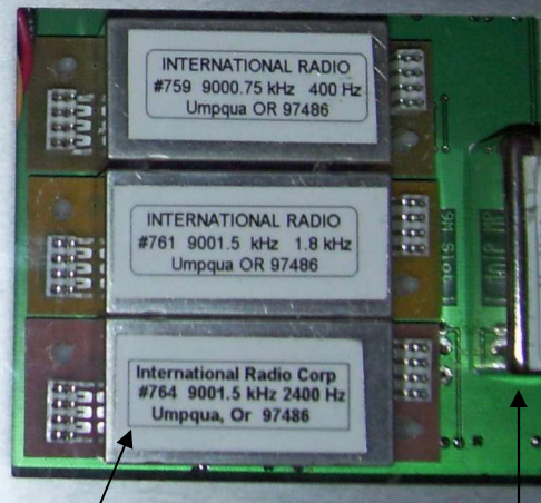
Photo K1: Typical filter installation
