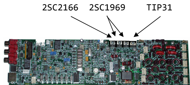
Transmitter board, top view
