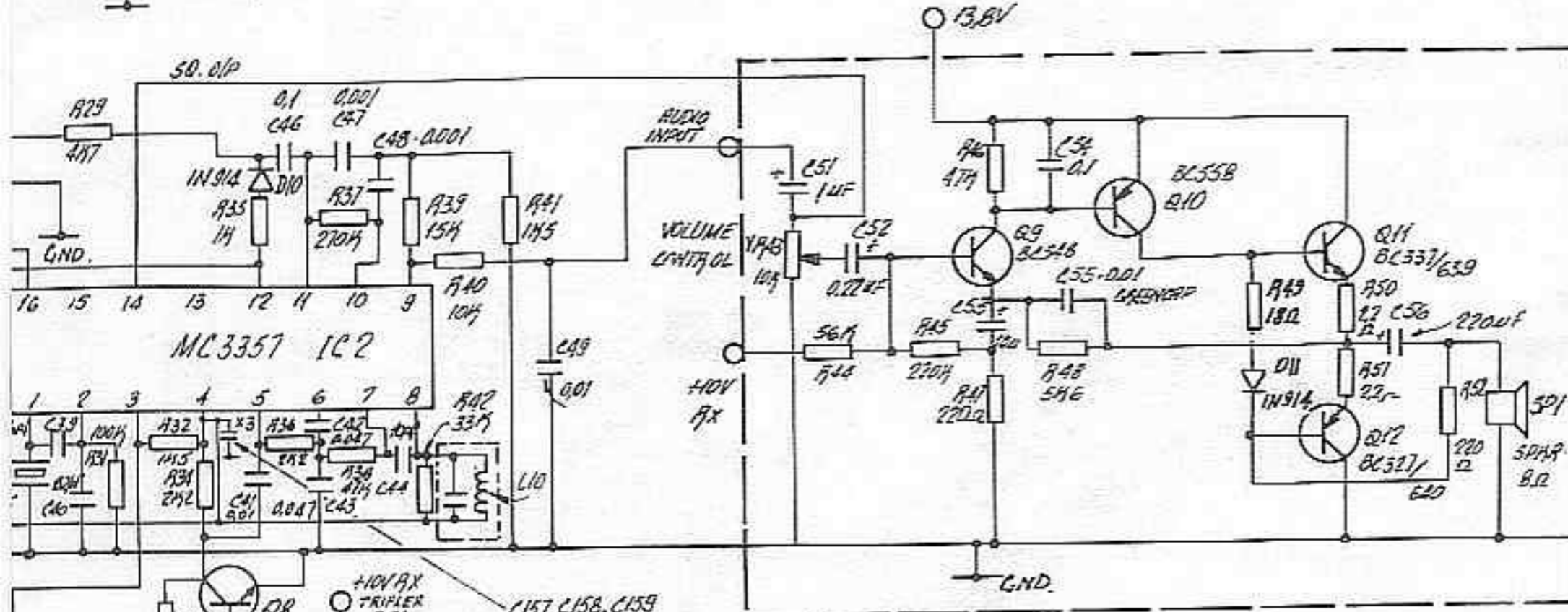
AUDIO AMP
