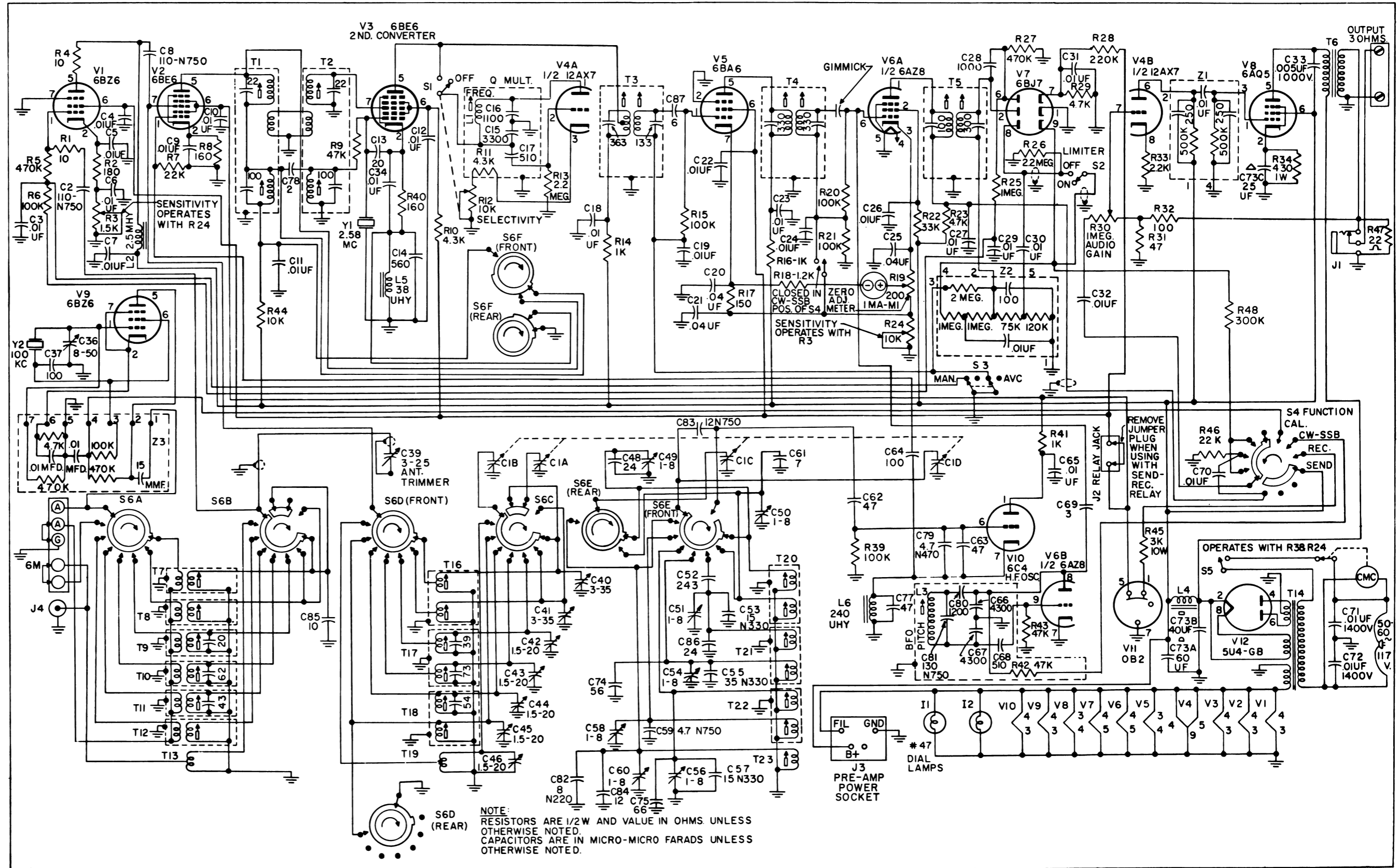
Figure 10. Hammarlund HQ-110A Communications Receiver, Schematic Diagram
