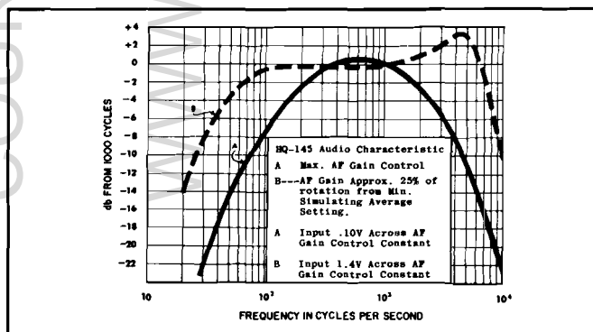
Figure 8. Auto Response Curve
