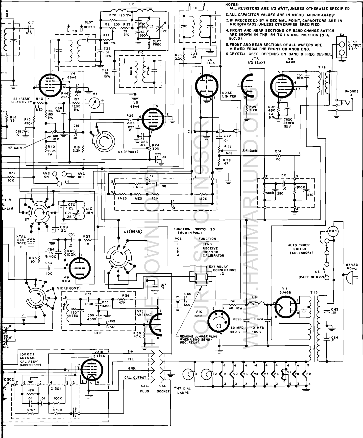
Figure 12. Hammarlund HQ-145X Communications Receiver, Schematic Diagram
