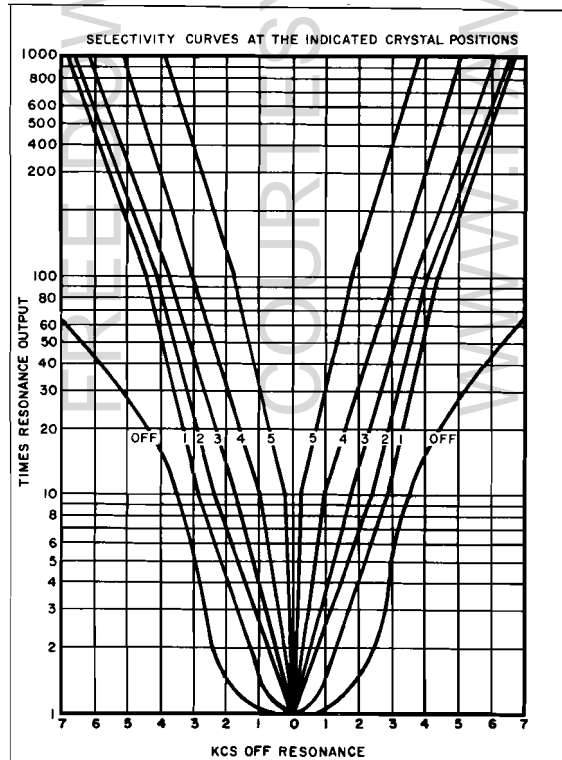
Figure 6. Selectivity Curves
