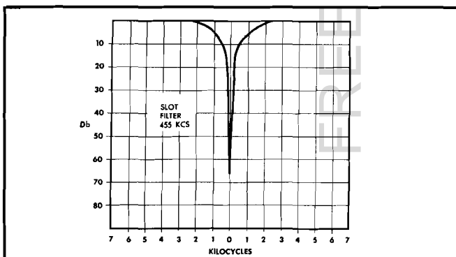
Figure 7. Slot Filter Response Curve
