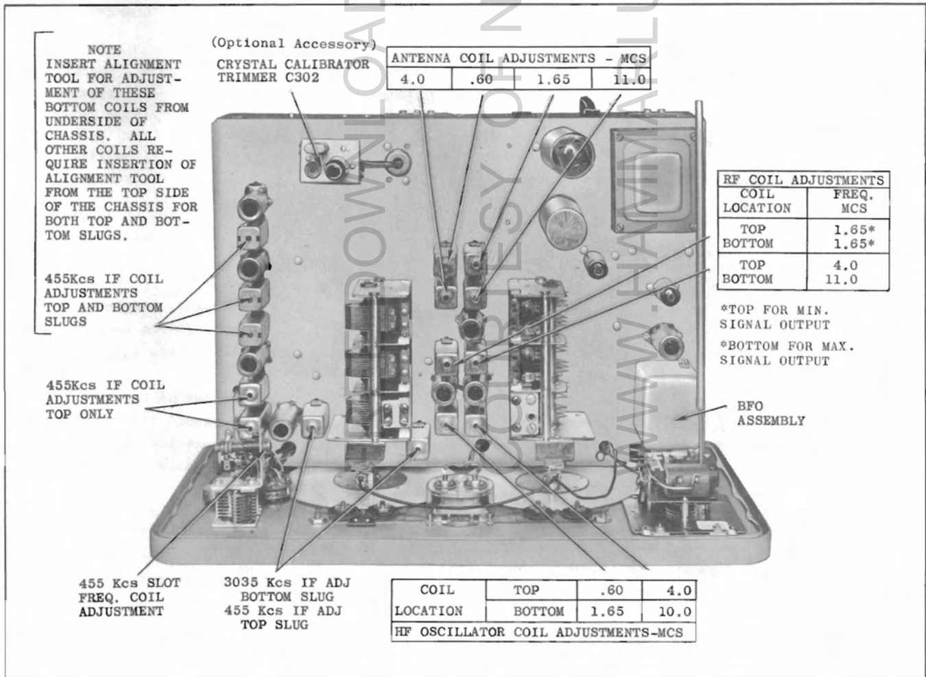
Figure 9. Top View of Chassis
