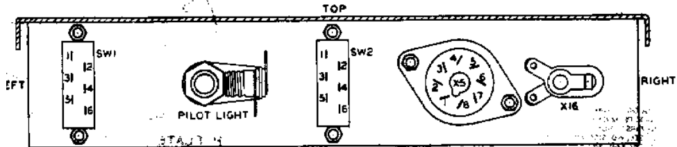
FRONT INSIDE CHASSIS LIP
