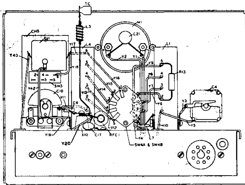
INSIDE BACK VIEW WITHOUT POWER TRANSFORMER "T" AND CHOKE "L1"
