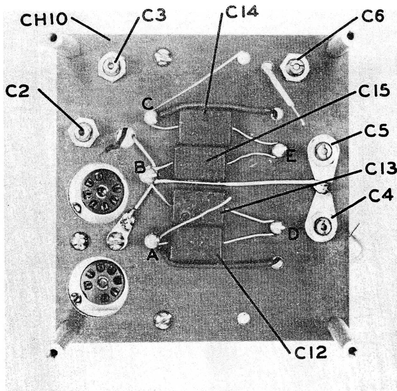
FIGURE 3A. V.F.O. CHASSIS TOP VIEW.
