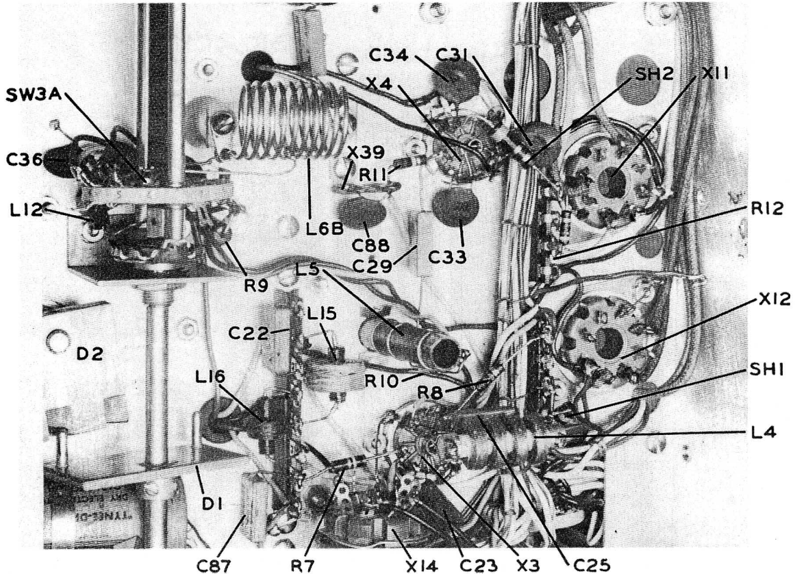
FIGURE 4B. R.F. EXCITER SECTION BOTTOM VIEW.
