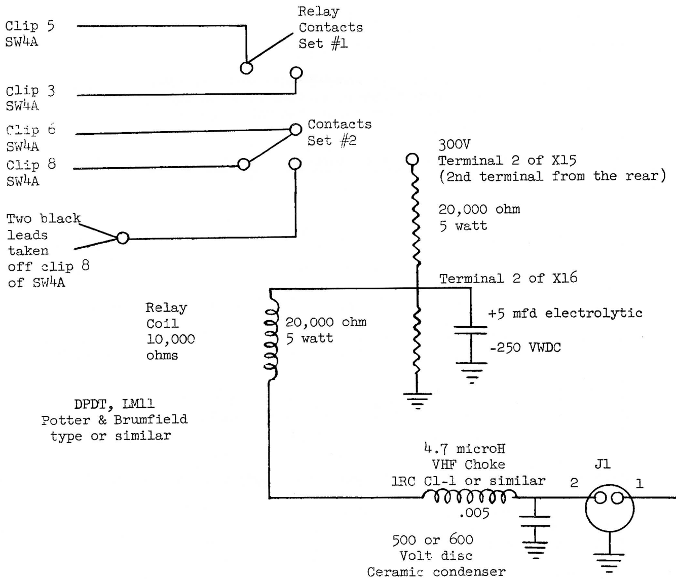
Schematic-Wiring Connections of the Push-to-Talk Circuit
