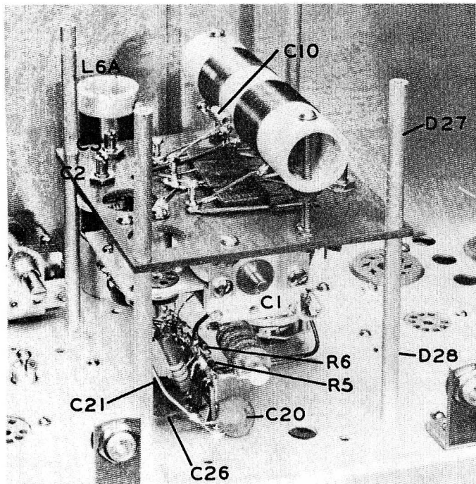
LEFT VIEW
