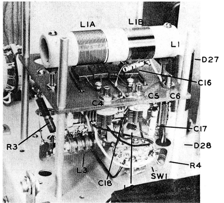
RIGHT VIEW.
