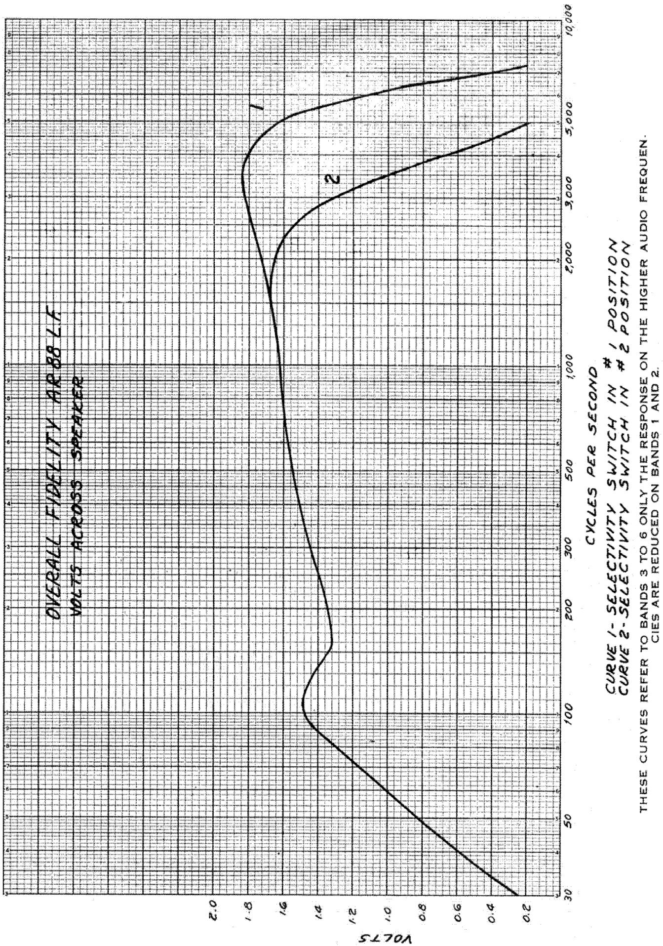
Figure 13.—General Purpose Communications Receiver—Fidelity Characteristics.
