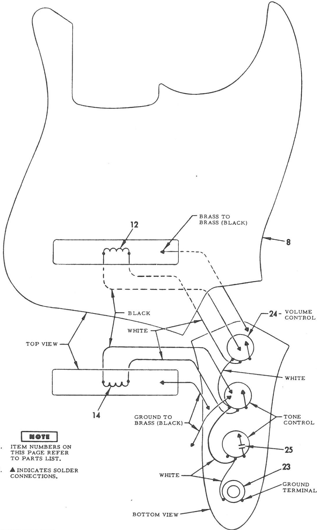
JAZZ BASS WIRING DIAGRAM
