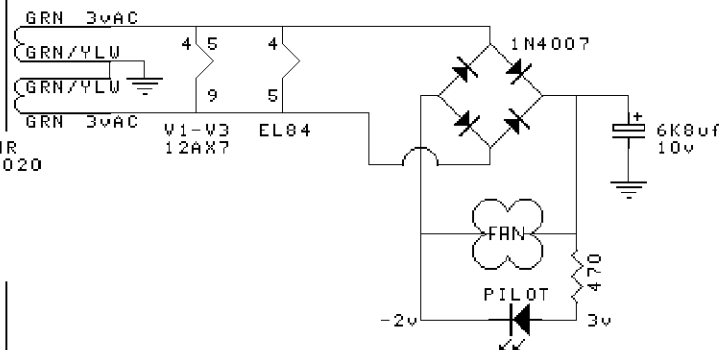
LOW V SUPPLIES
