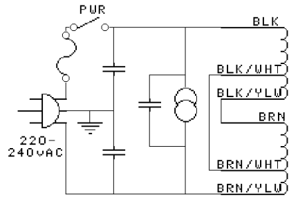
EXPORT PRIMARY XFMR #561020
