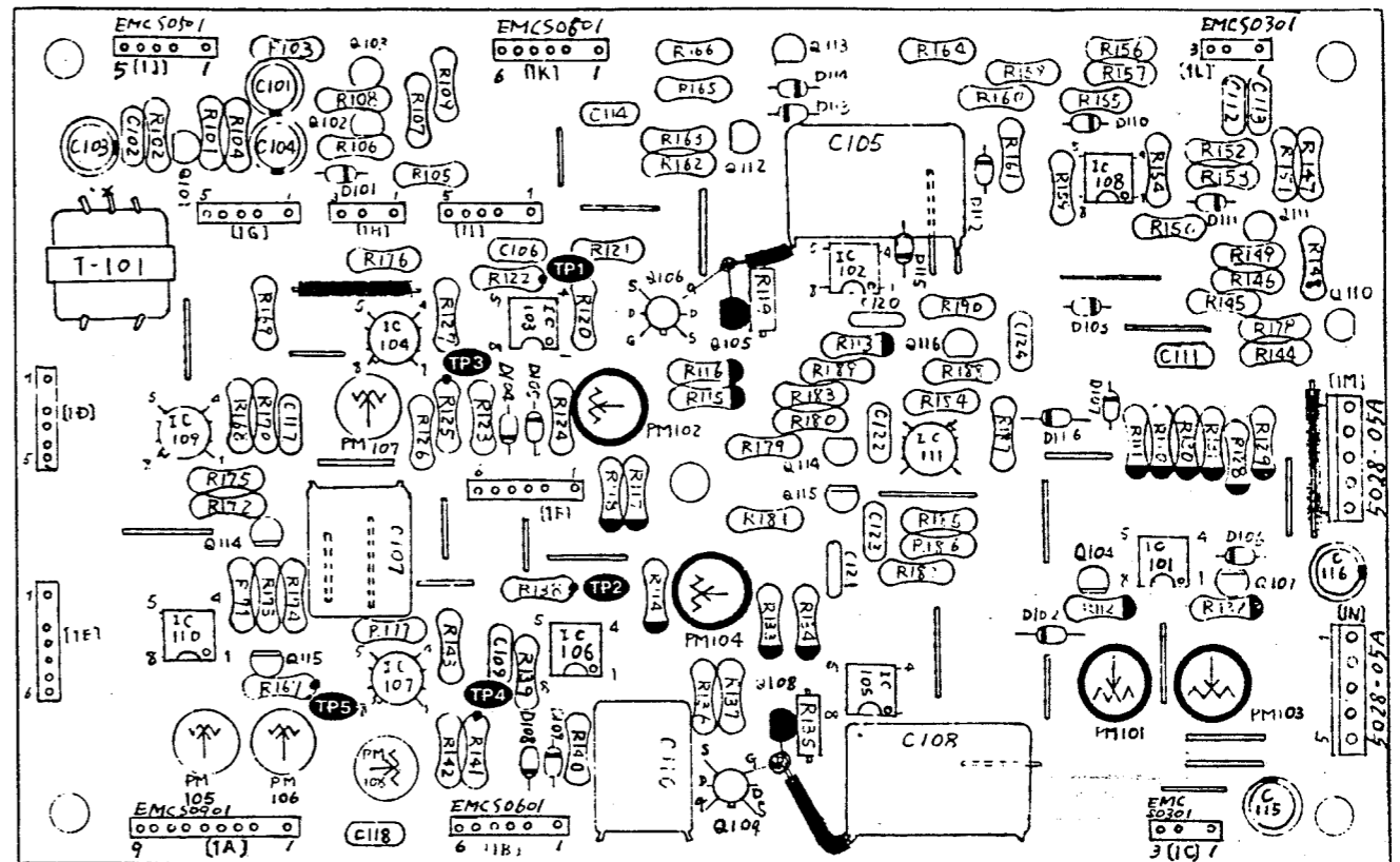
CVH-1A (159H001A) (SERIAL NO. 700550 AND HIGHER)
