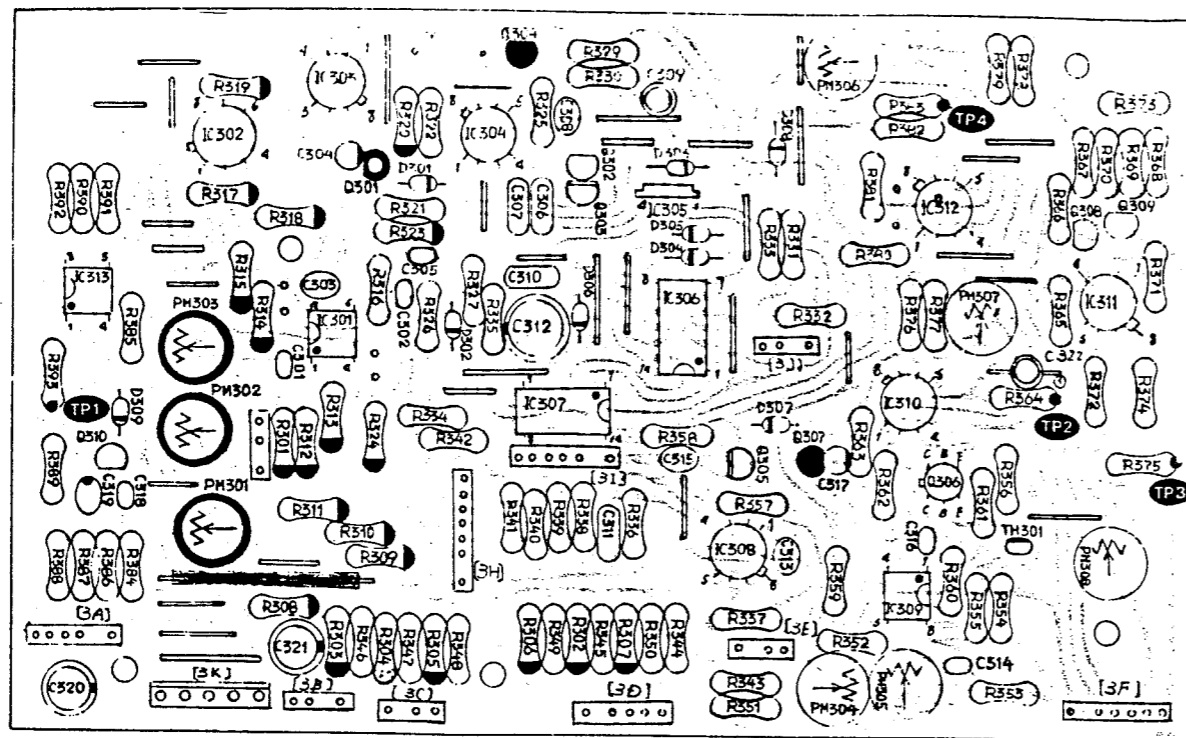
VCOH-1 - PARTS ON THE FOIL SIDE
