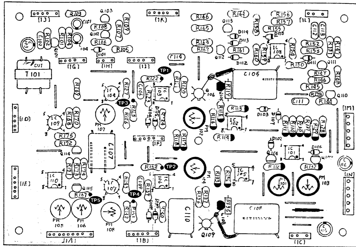
CVH-1 - PARTS ON THE FOIL SIDE
