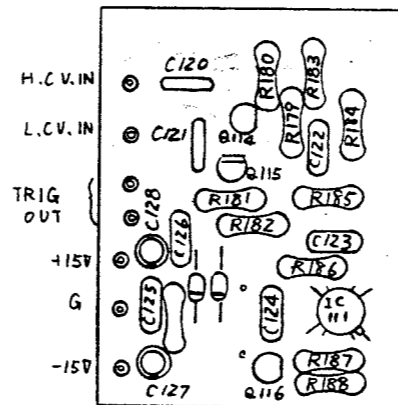
PARTS ON THE FOIL SIDE
