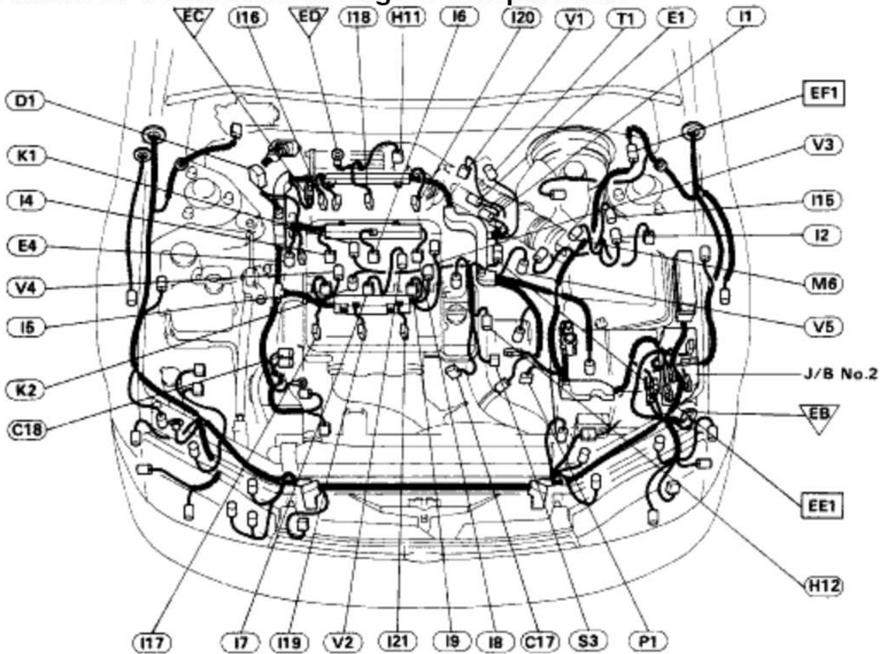
C17 Camshaft Position Sensor
