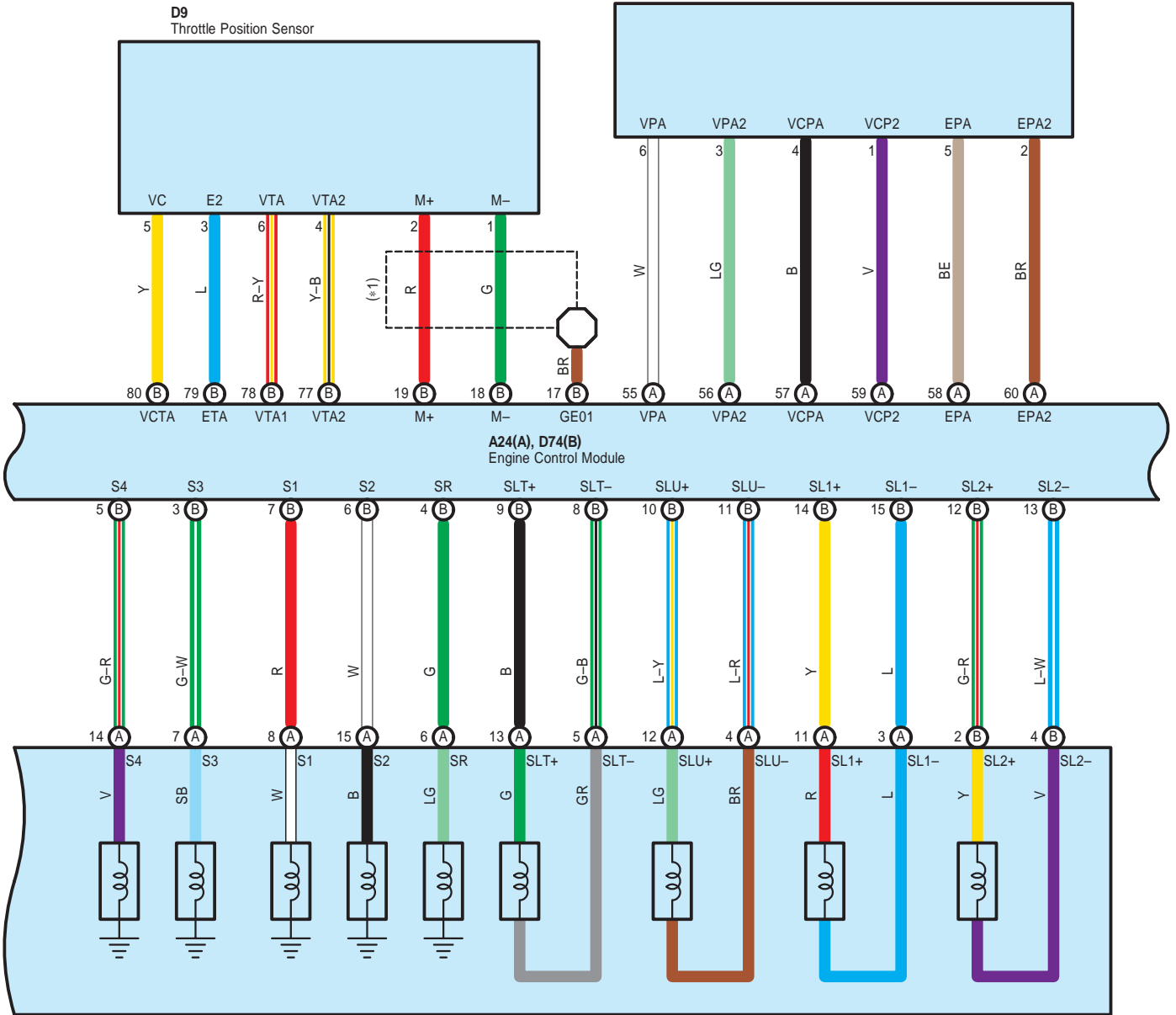
D63(A), D64(B) Automatic Transmission
