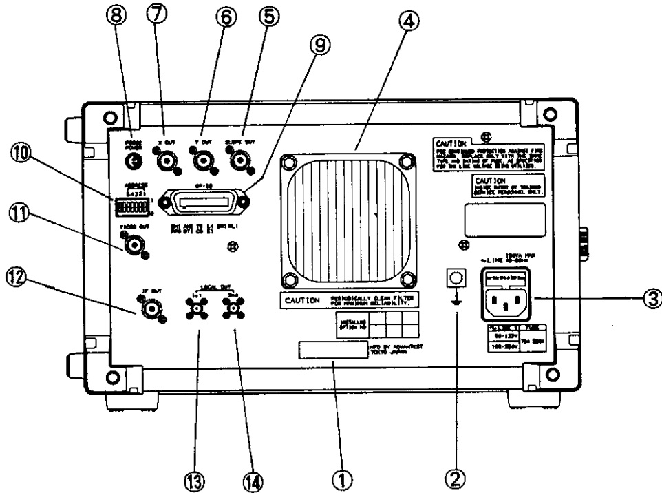
Figure 3-4 Rear Panel
