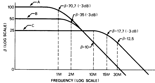
Fig. 15. β versus frequency for transistors A, B and C.
