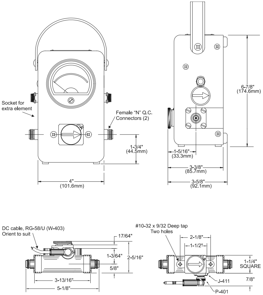
Figure 2 Bird 43 Thru-line Wattmeter Outline Drawing
