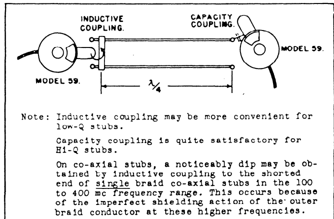
Figure 11 - COUPLING TO QUARTER-WAVE STUBS
