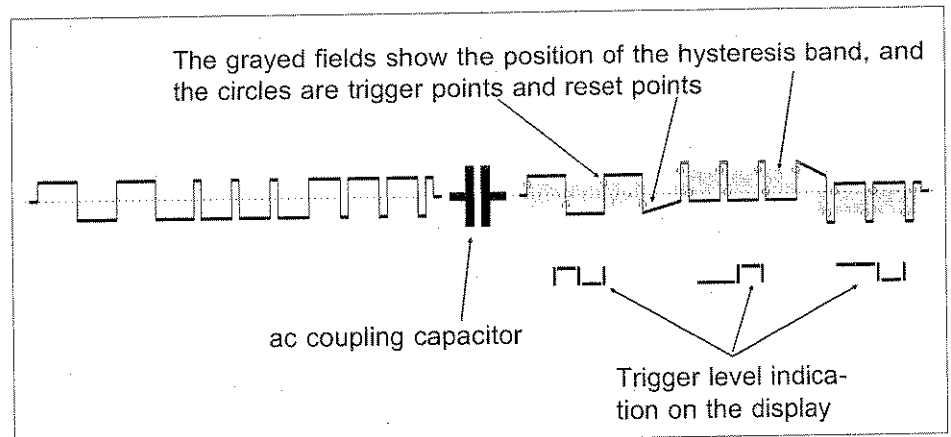
Dc shift caused by the ac coupling capacitor.
