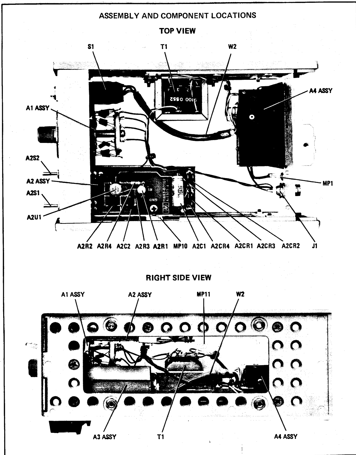
Figure 13. 11683A Assembly and Component Locations
