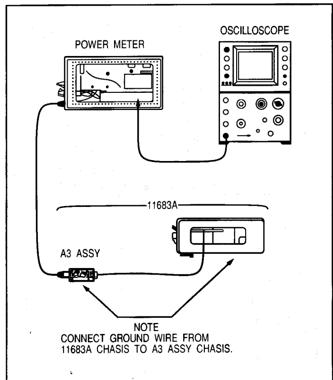
Figure 9. FET Balance Adjustment Setup
