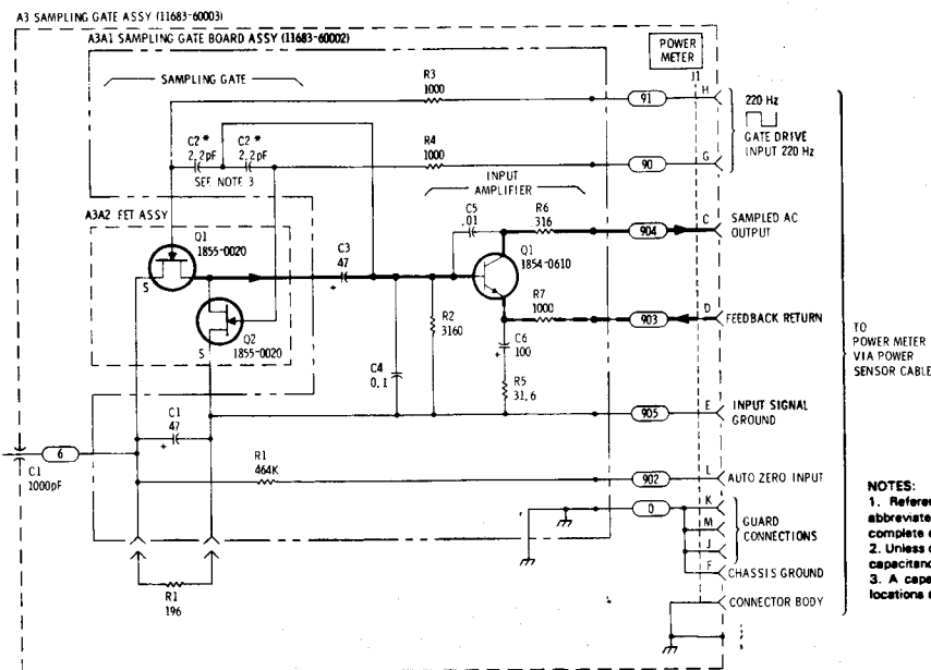
Figure A3. Range Switch/Sampling Gate Schematic Diagram (P/O Figure 18)
