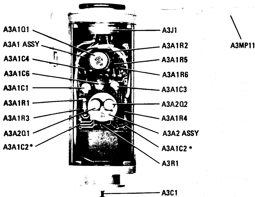
Figure A2. Assembly Component Locations
