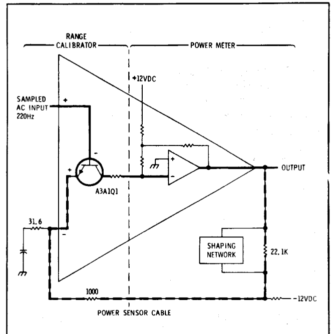
Figure 12. Hybrid Operational Amplifier
