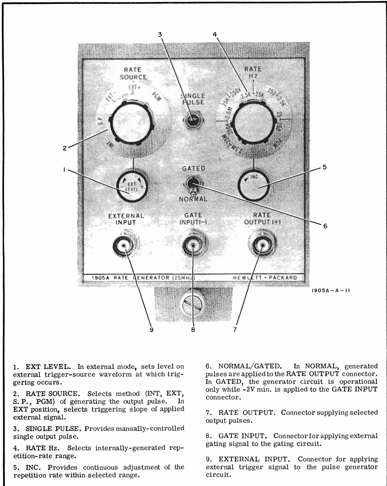
Figure 3-1. Front-panel Controls and Connectors.
