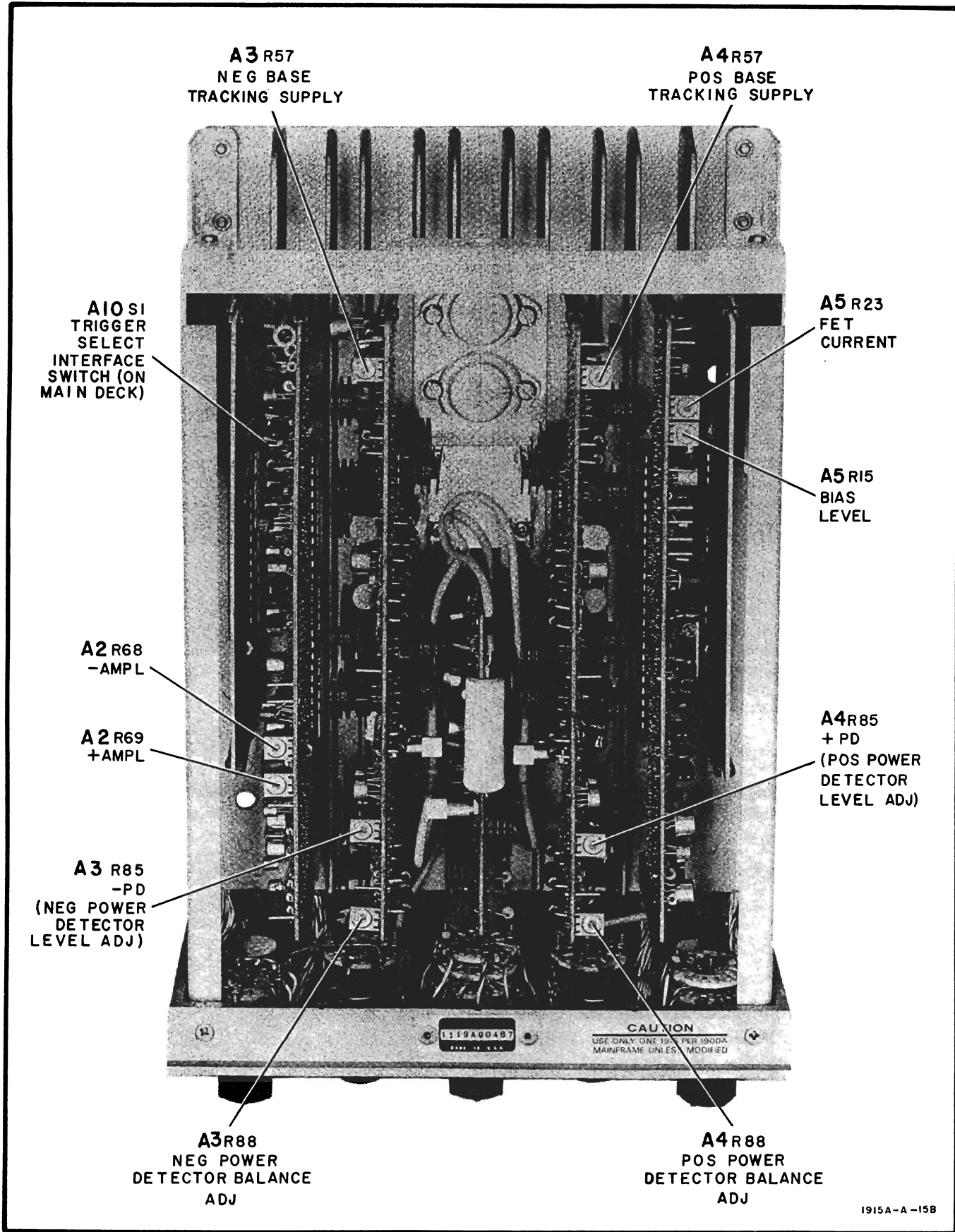
Figure 8-1. Adjustment Locations
