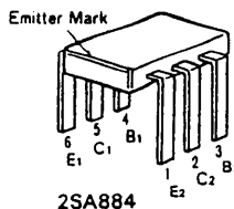
2SA884
