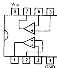
NJM4558D
