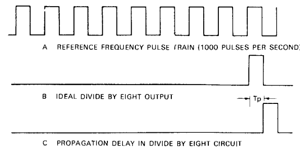
Fig. 3 Waveforms in divide-by-eight circuit
