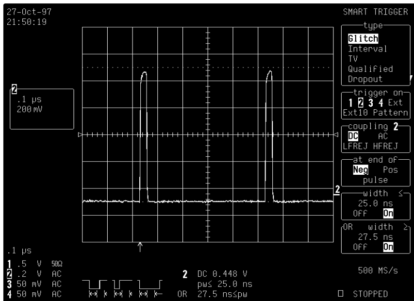
Figure 8-8. Exclusion Trigger. Only pulses within or outside the boundaries of the width range are captured.
