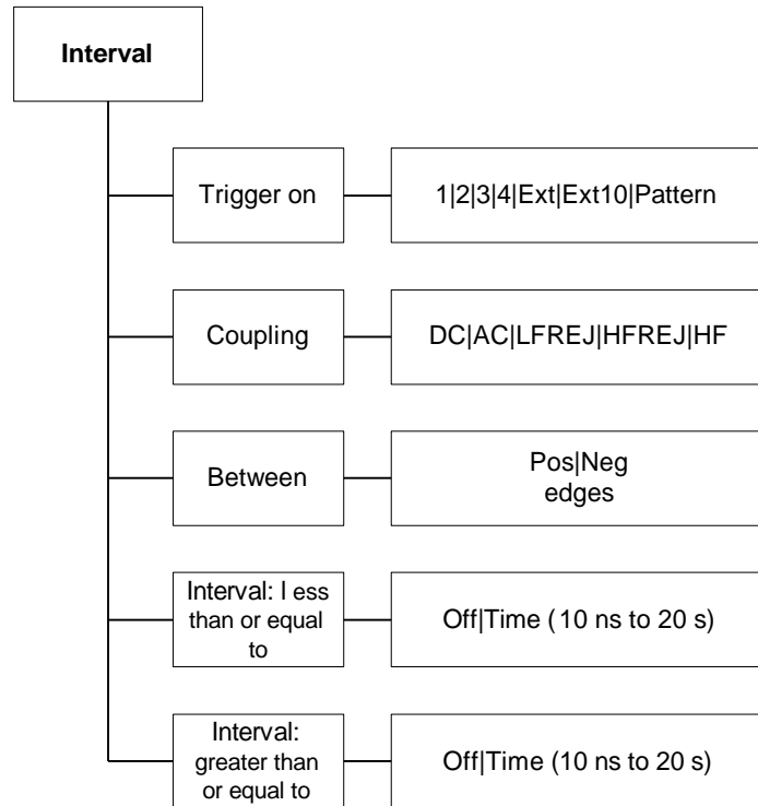
Figure 8–9. Interval Trigger Menu (see page 8–32).
