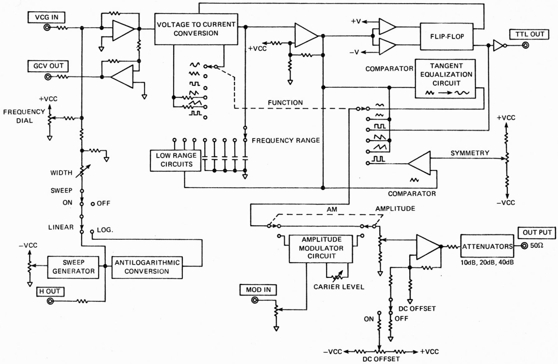
MODEL LFG 1300 FUNCTION GENERATOR
