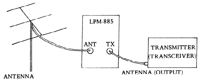
Fig. 2-1 Interconnections.
