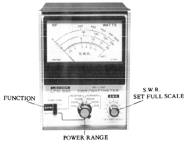
Fig. 1-1 Front panel functions.
