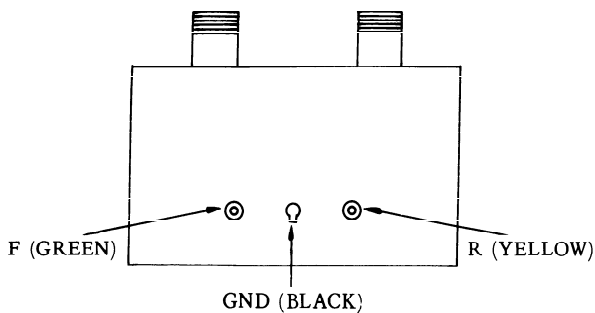
Fig. 2-4 Top view of the detector unit.
