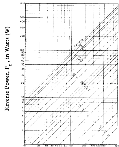
Fig. 2-2 SWR nomograph.
