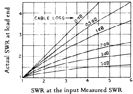
Fig. 2-3 Correction curves for cable loss.
