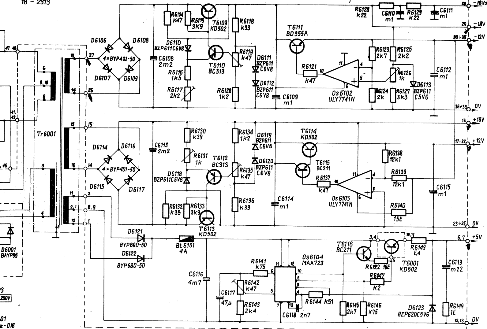
ZASILACZ POWER SUPPLY OT-327
