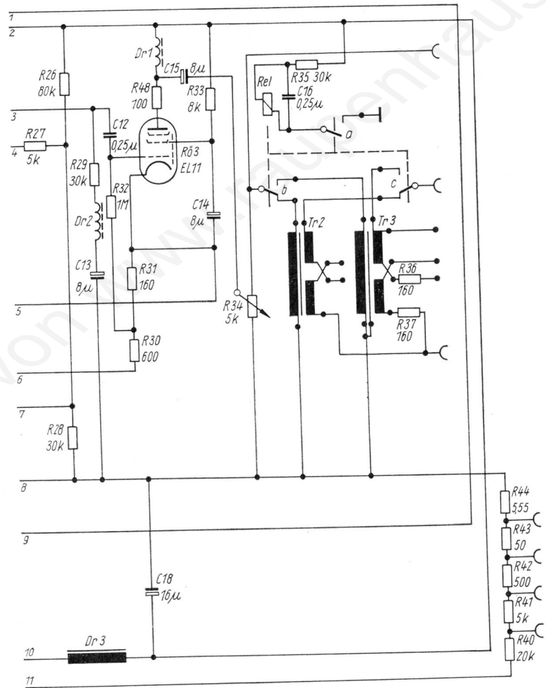
RC-Generator GF 8
