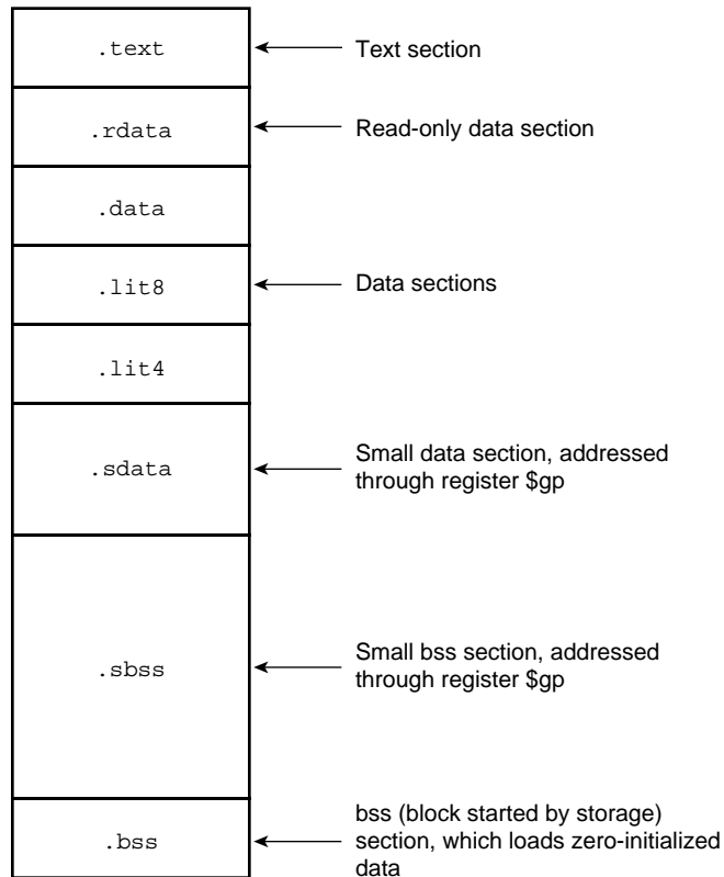
Figure 1. Section and Location Counters
