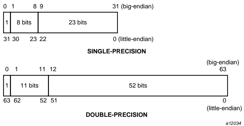
Figure 2. Floating Point Formats
