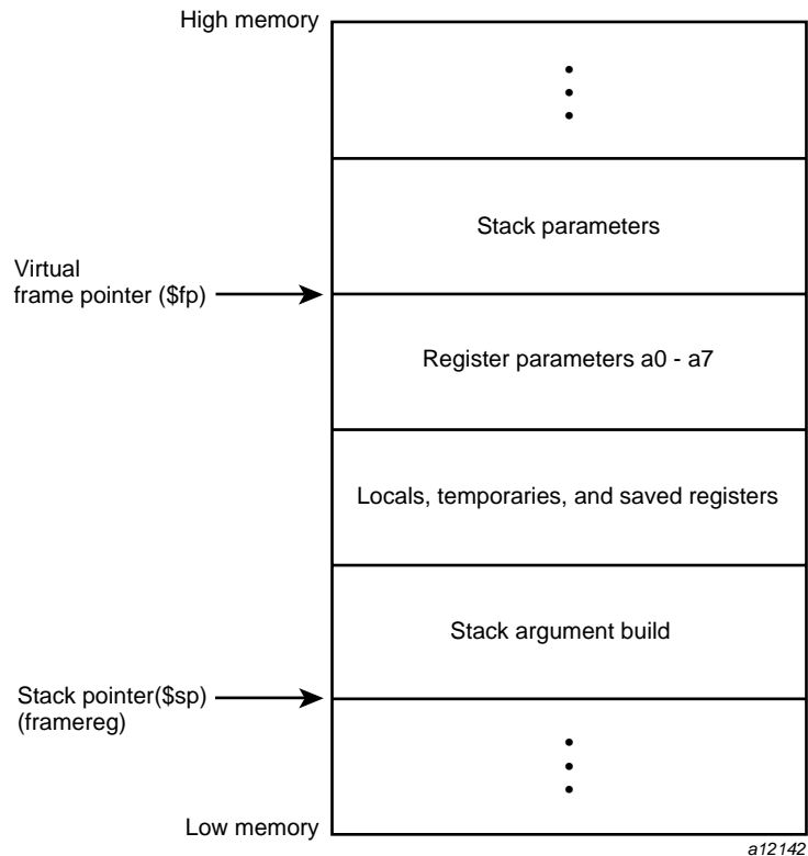
Figure 5. Stack Organization for -n32 and -64
