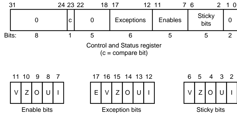
Figure 3. Floating Control and Status Register 31
