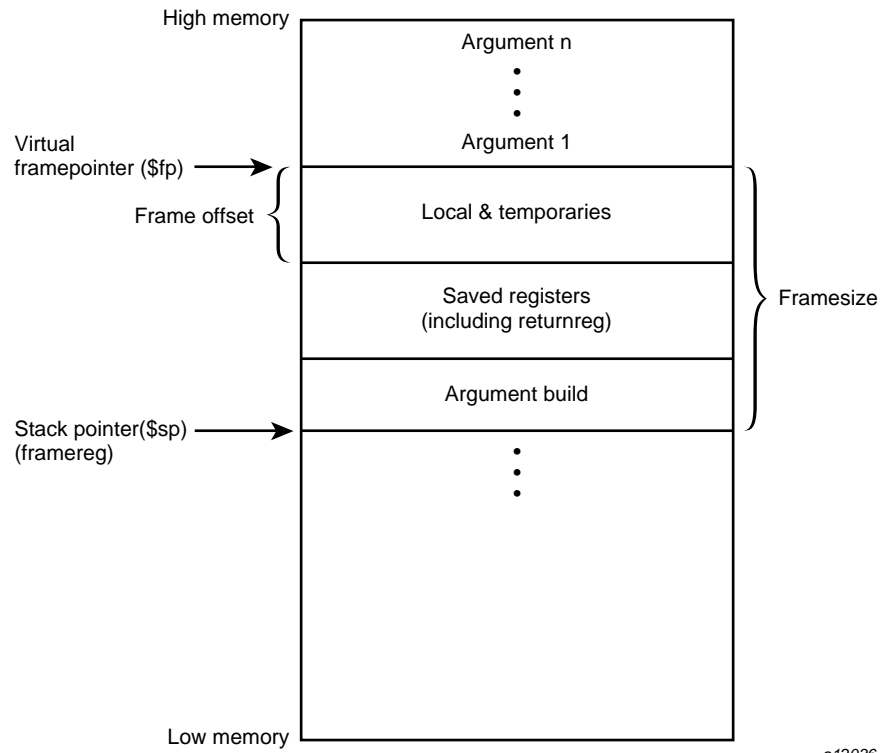
Figure 4. Stack Organization for -32
