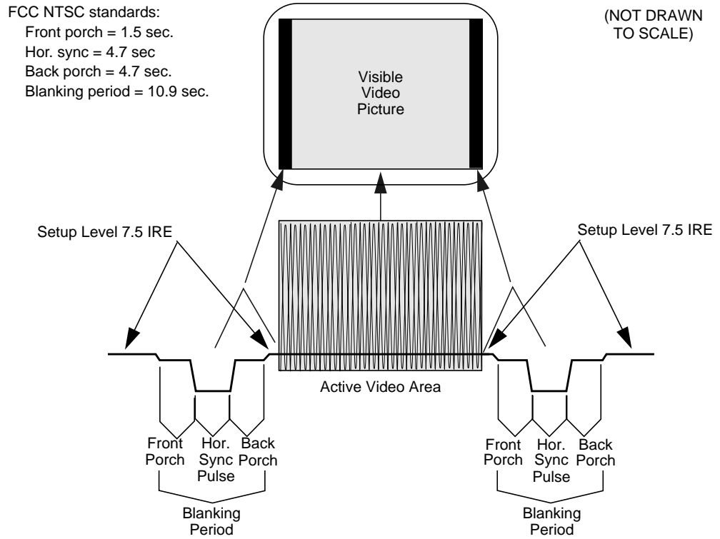
Figure GI-4 Horizontal Blanking
