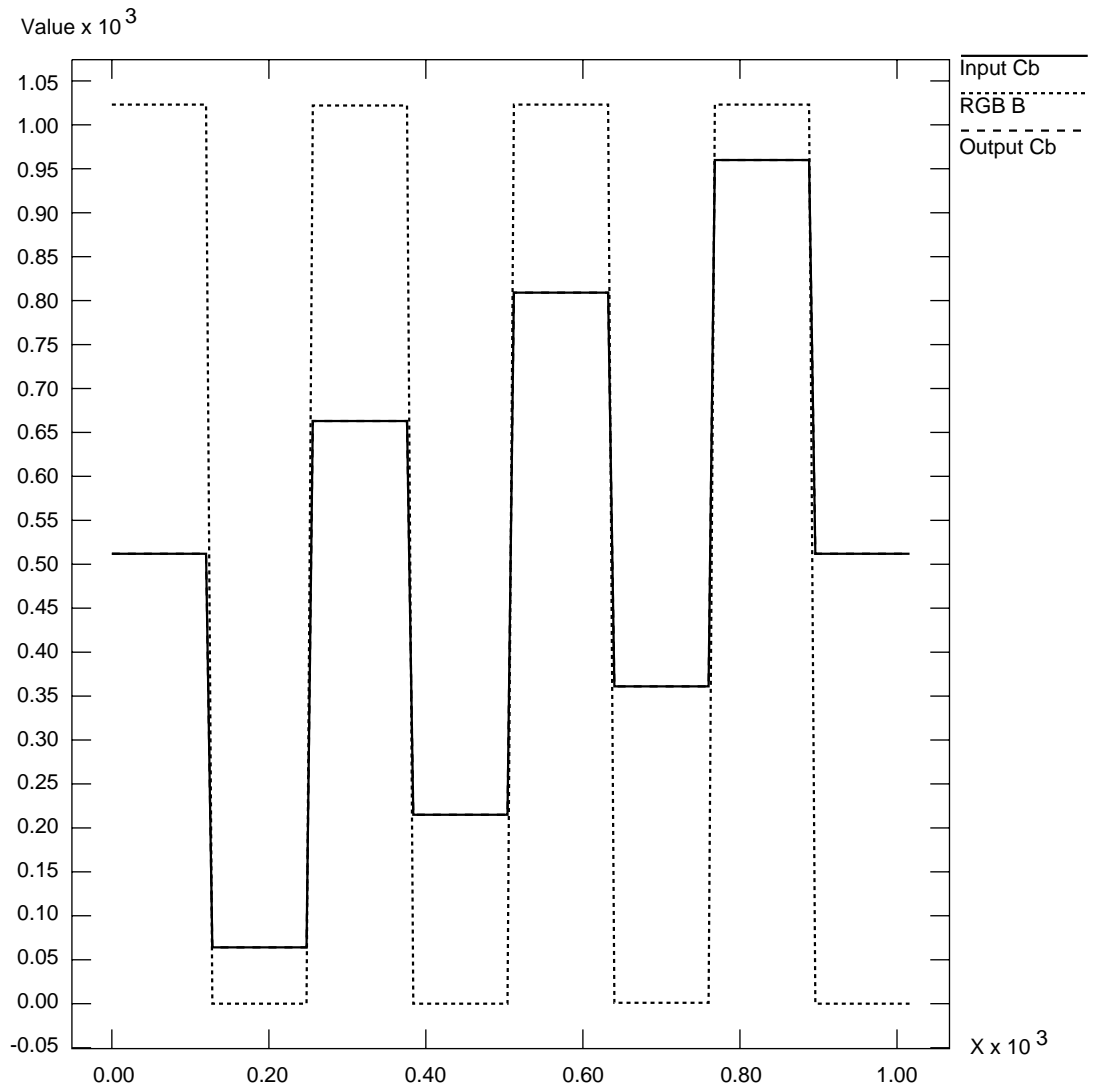
Figure D-5 100% Color Bars: Cb/B
