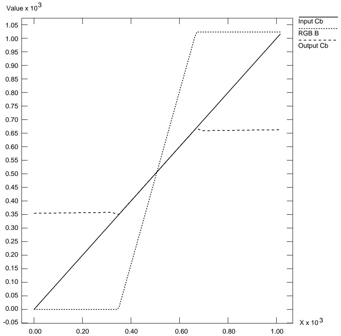
Figure D-11 Chroma/Luma Ramp: Cb/B
