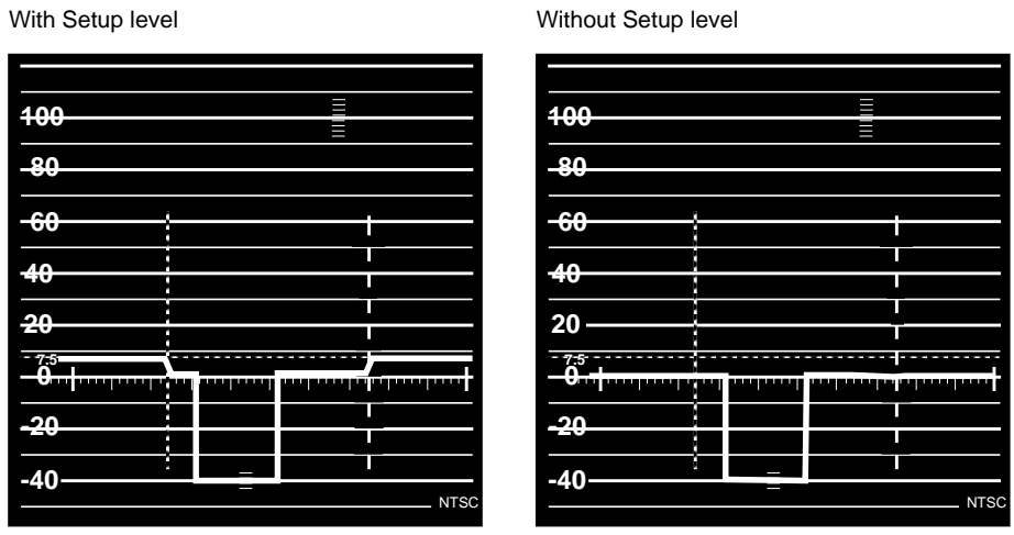
Figure G1-6 Waveform Monitor Readings With and Without Setup
