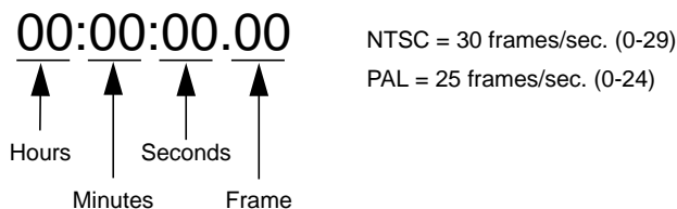
Figure G1-7 SMPTE Time Code
