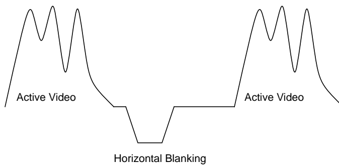
Figure GI-9 Y or Green Plus Sync Signal
