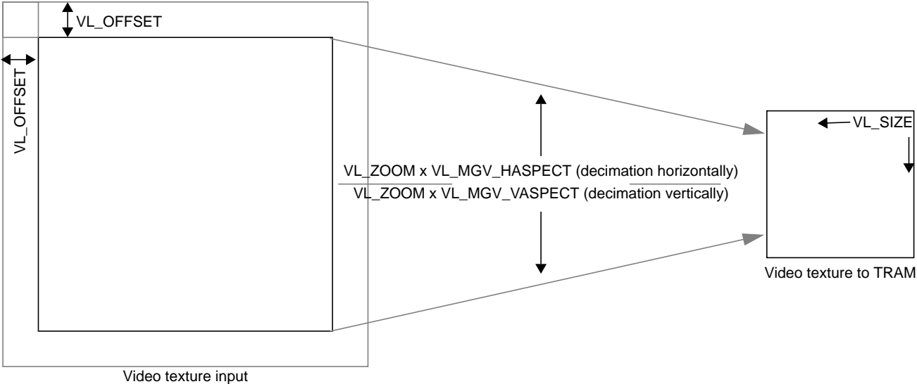
Figure 9-5 Zoom, Size, and Offset for Video Texture Mapping
