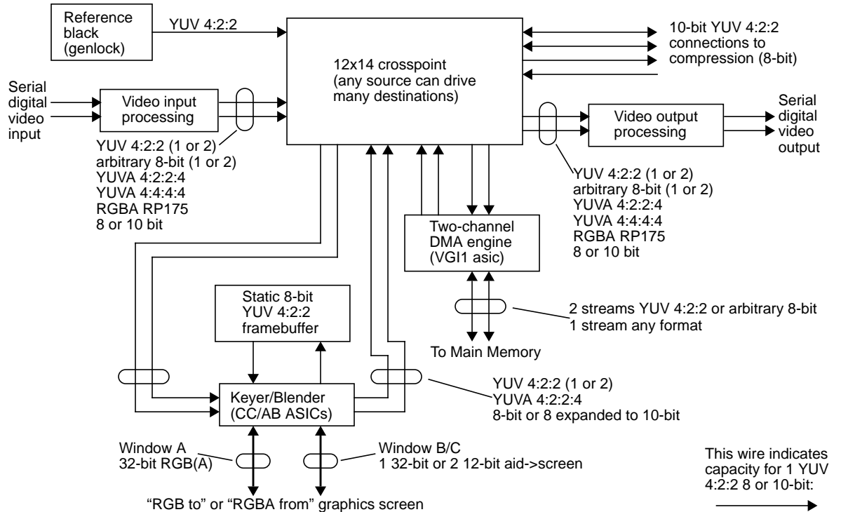
Figure 5-1 Hardware Representation
