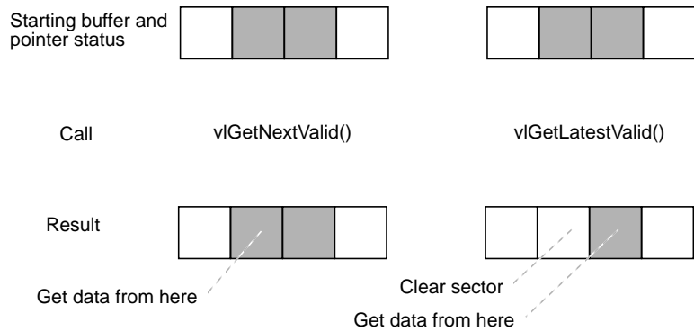
Figure 2-4 vlGetNextValid() , vlGetLatestValid() , and vlPutFree()
