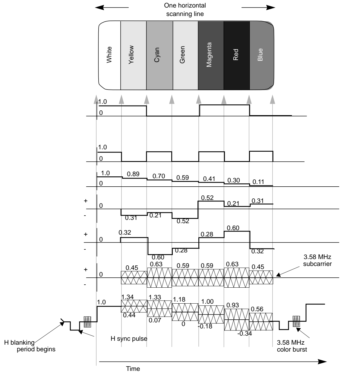
Figure GI-3 Component Video Signals
