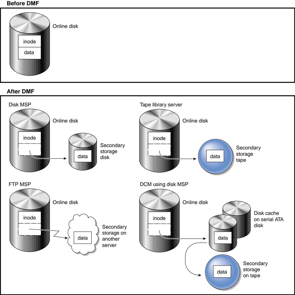
Figure 1-2 DMF Mechanisms
