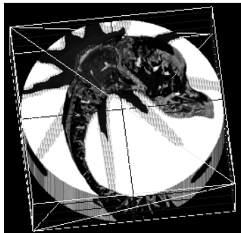
Figure 6-4 Overlapping Volumes
