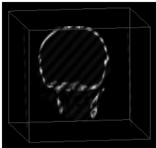
Figure 6-7 MPR Bands
