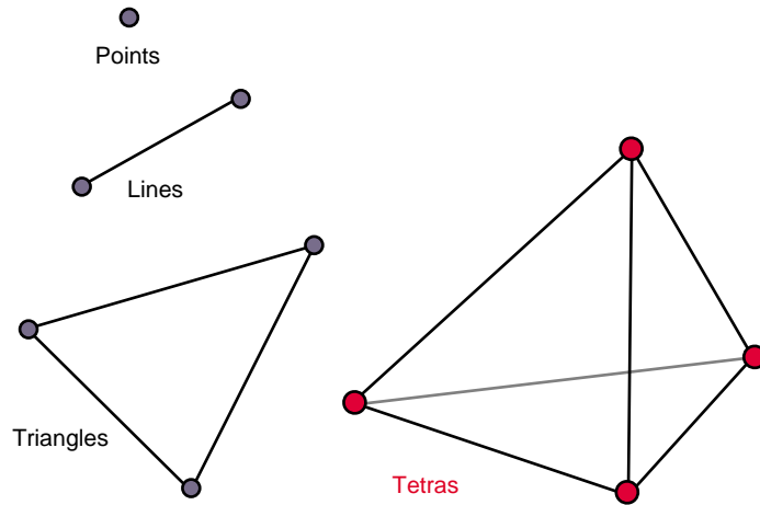
Figure 2-1 Geometric Primitives
