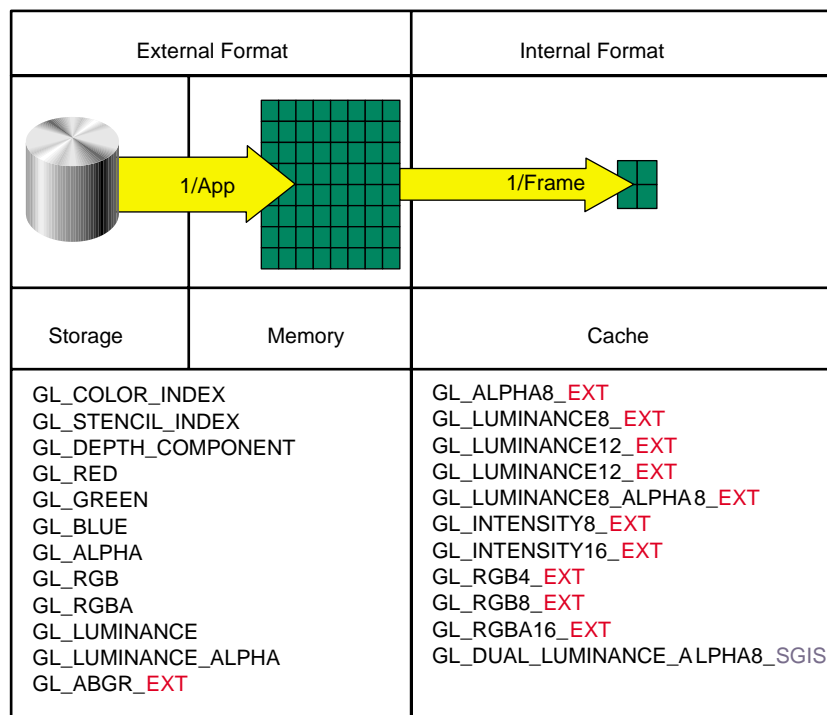
Figure 7-1 Data Formats
