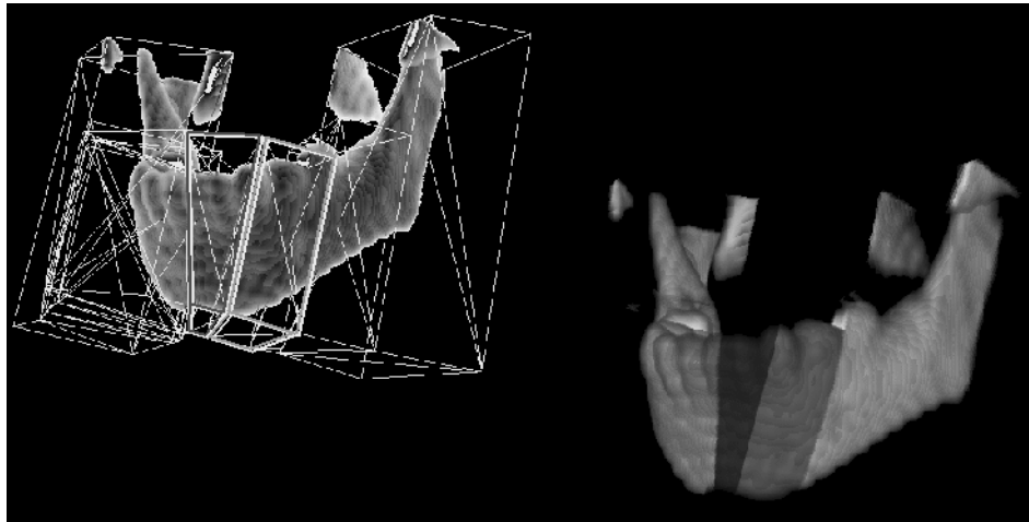
Figure 2-7 Per-part Properties.
