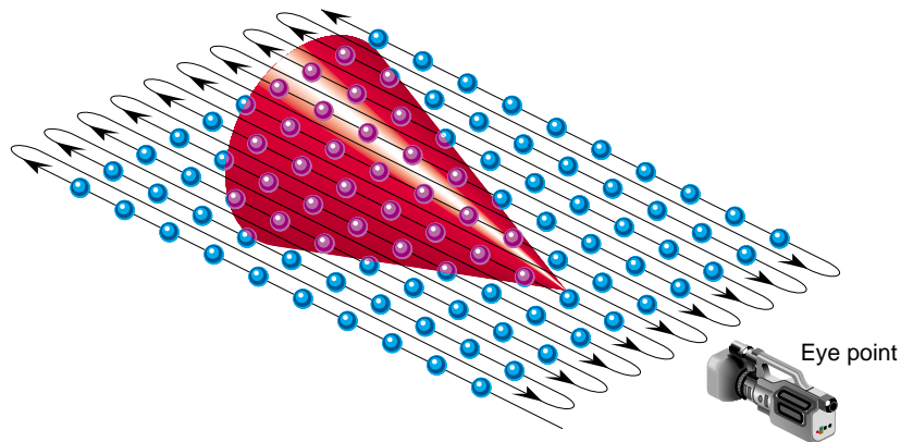
Figure 2-14 Ray Casting Processing order
