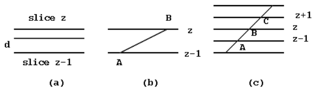
Figure 6-6 MPR with Two-Dimensional Texture Mapping
