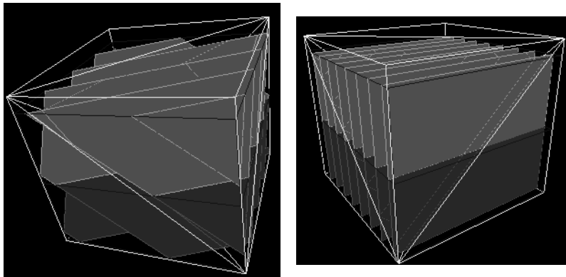
Figure 3-5 A Volume Polygonized Using VIEWPORT_ALIGNED and AXIS_ALIGNED Sampling
