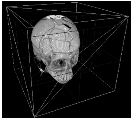
Figure 2-17 Brick Set
