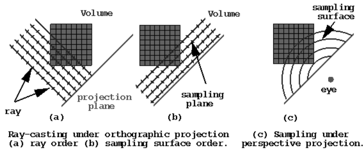
Figure 2-12 Processing Order
