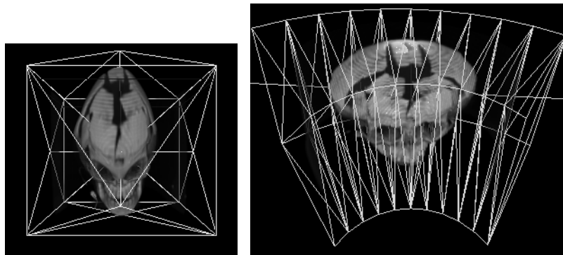
Figure 2-5 Volume Deformation
