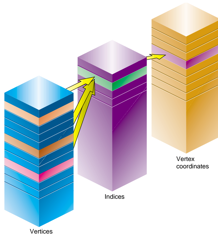
Figure 3-2 Indexed Vertices
