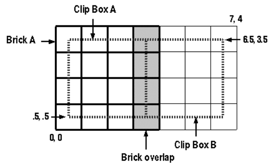
Figure 2-19 Brick Overlap
