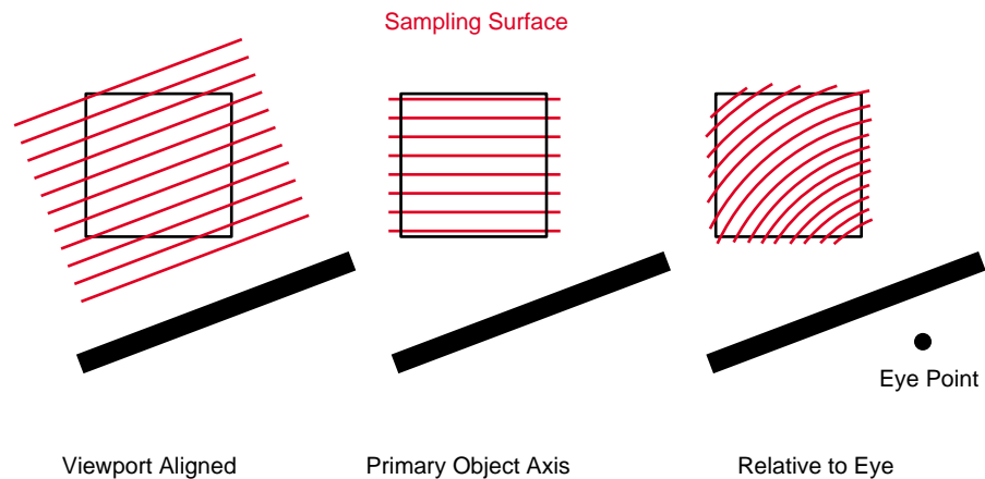
Figure 3-4 Sampling Surface
