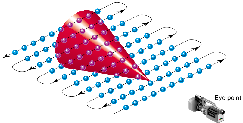
Figure 2-15 Volume Slicing
