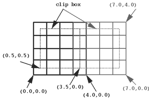
Figure 2-20 Bricks Overlapping
