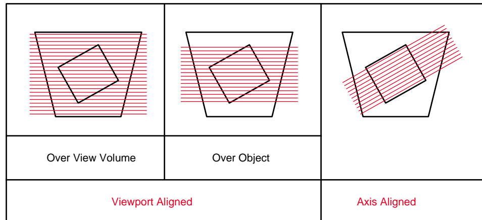
Figure 3-6 Sampling Spaces
