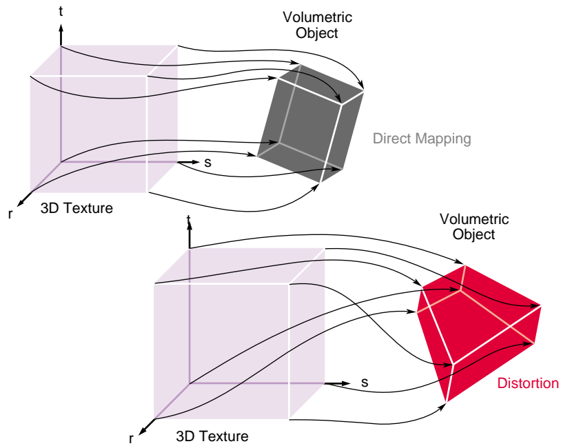
Figure 7-2 Voxel Coordinates
