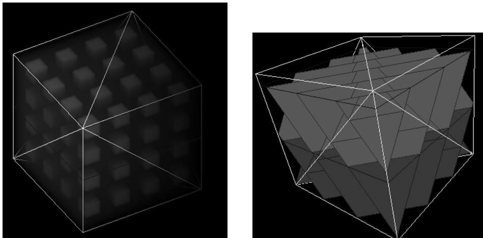
Figure 2-3 Colored Cubes
