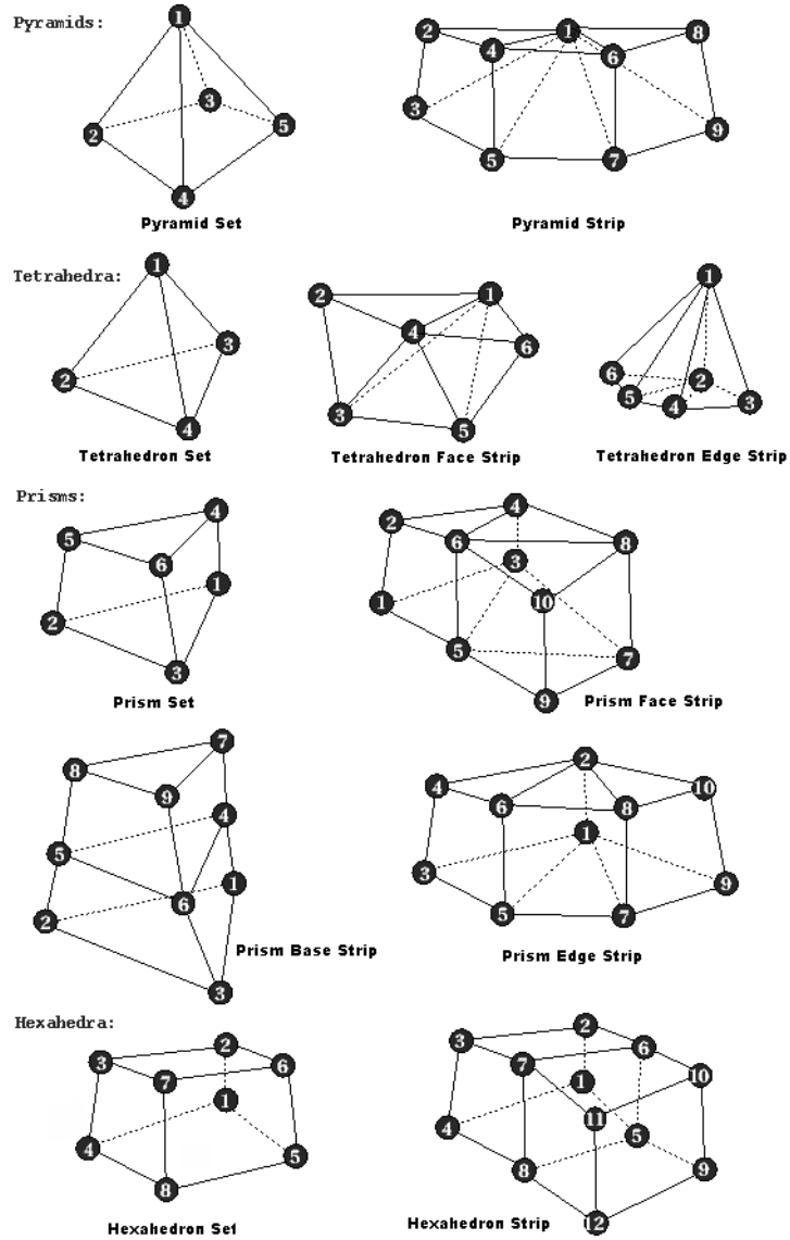
Figure 2-11 Volumetric Primitives
