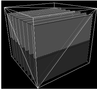
Figure 3-3 voFaceSets
