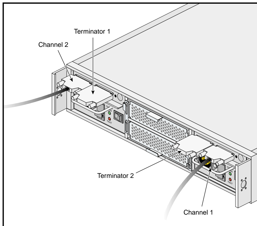
Figure 2-2 Attaching Interface Cable on 2 x 4 Configuration
