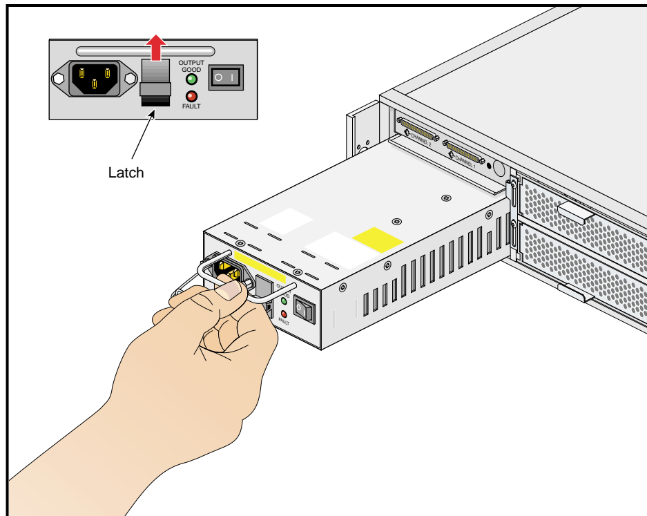
Figure 3-2 Power Supply Latch and Handle
