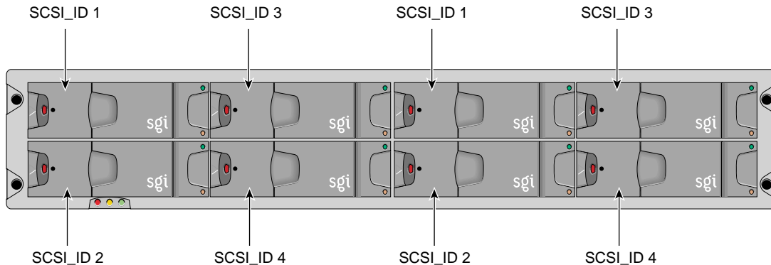
Figure 2-4 2 x 4 SCSI_ID Addressing
