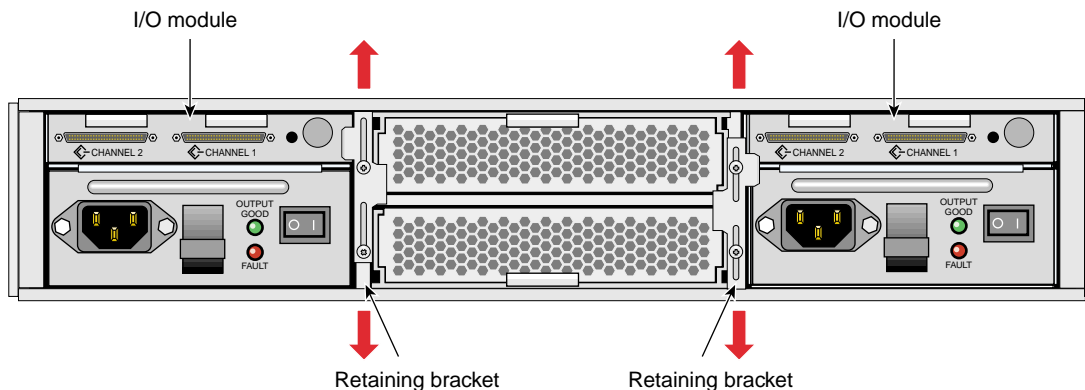
Figure 3-4 I/O Module Retaining Bracket
