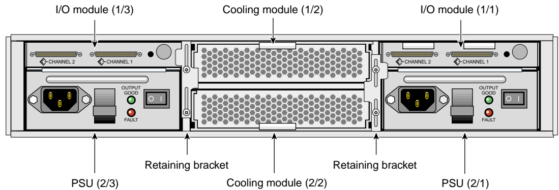
Figure 1-15 Rear Module Locations and Bay Numbering
