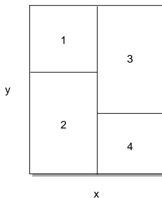
Figure 3-21 2D Tiling Scheme with Four Regions and Vertical Tiles
