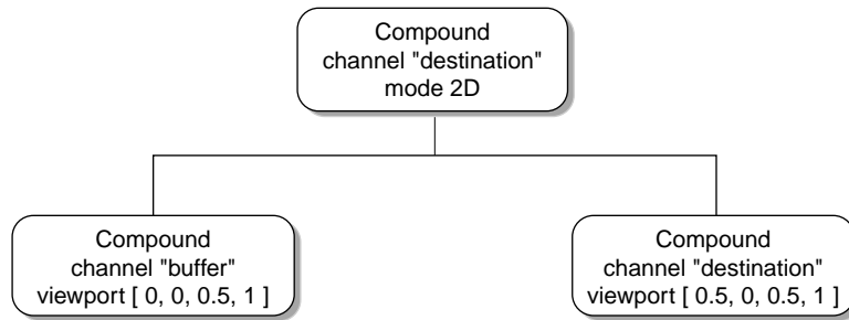
Figure 4-1 Compound Tree for a 2D Decomposition
