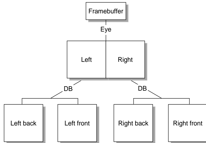
Figure 3-18 Eye-DB Multilevel Decomposition
