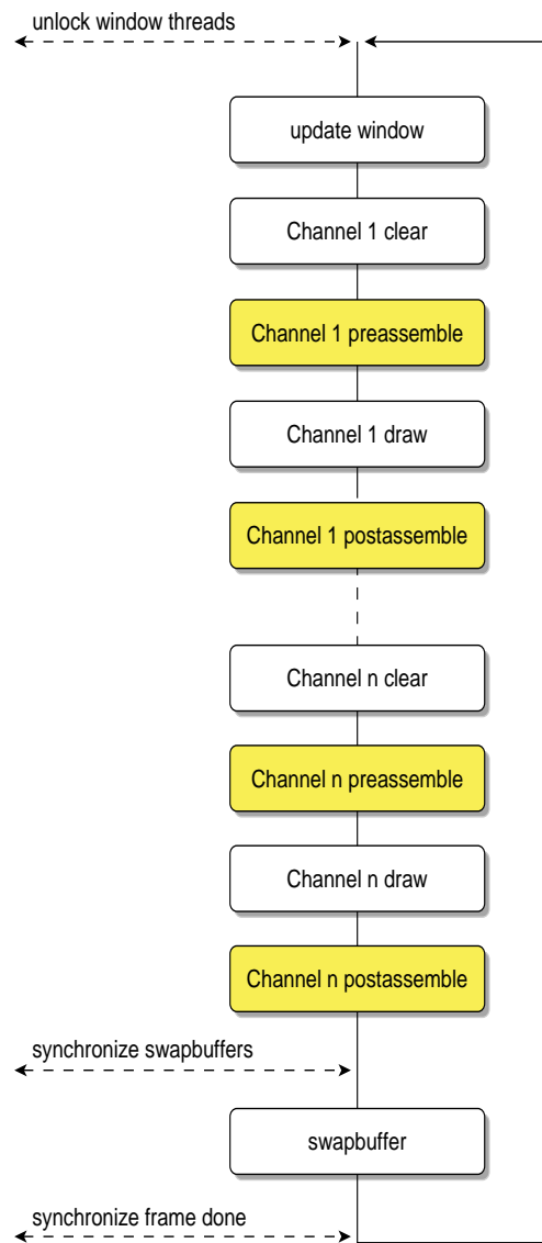
Figure 3-22 A Detailed Window Update
