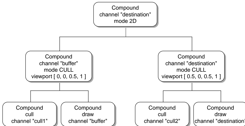
Figure 4-2 Compound Tree for 2D Decomposition with Parallel Culling
