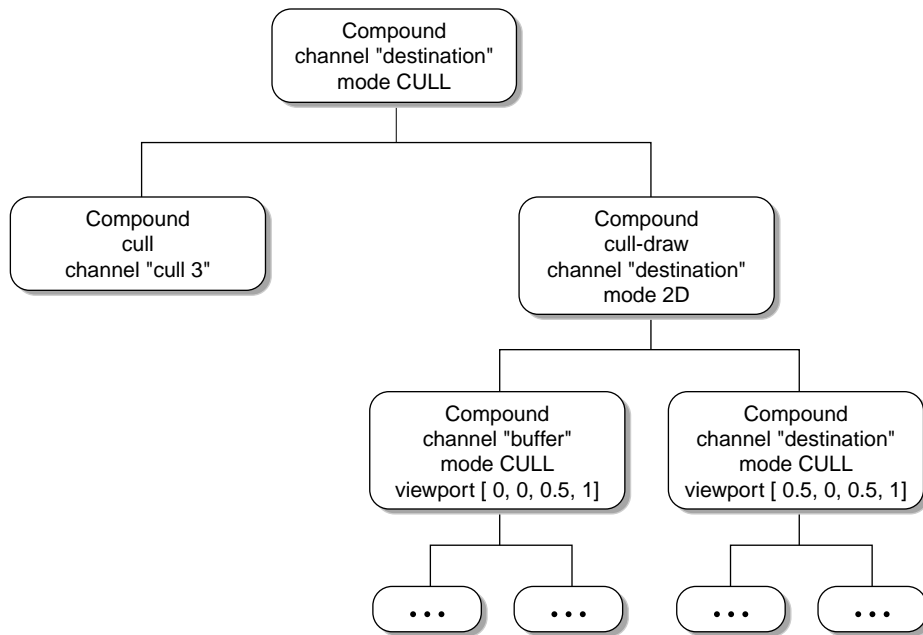
Figure 4-3 Compound Tree for 2D Decomposition and Multilevel Culling
