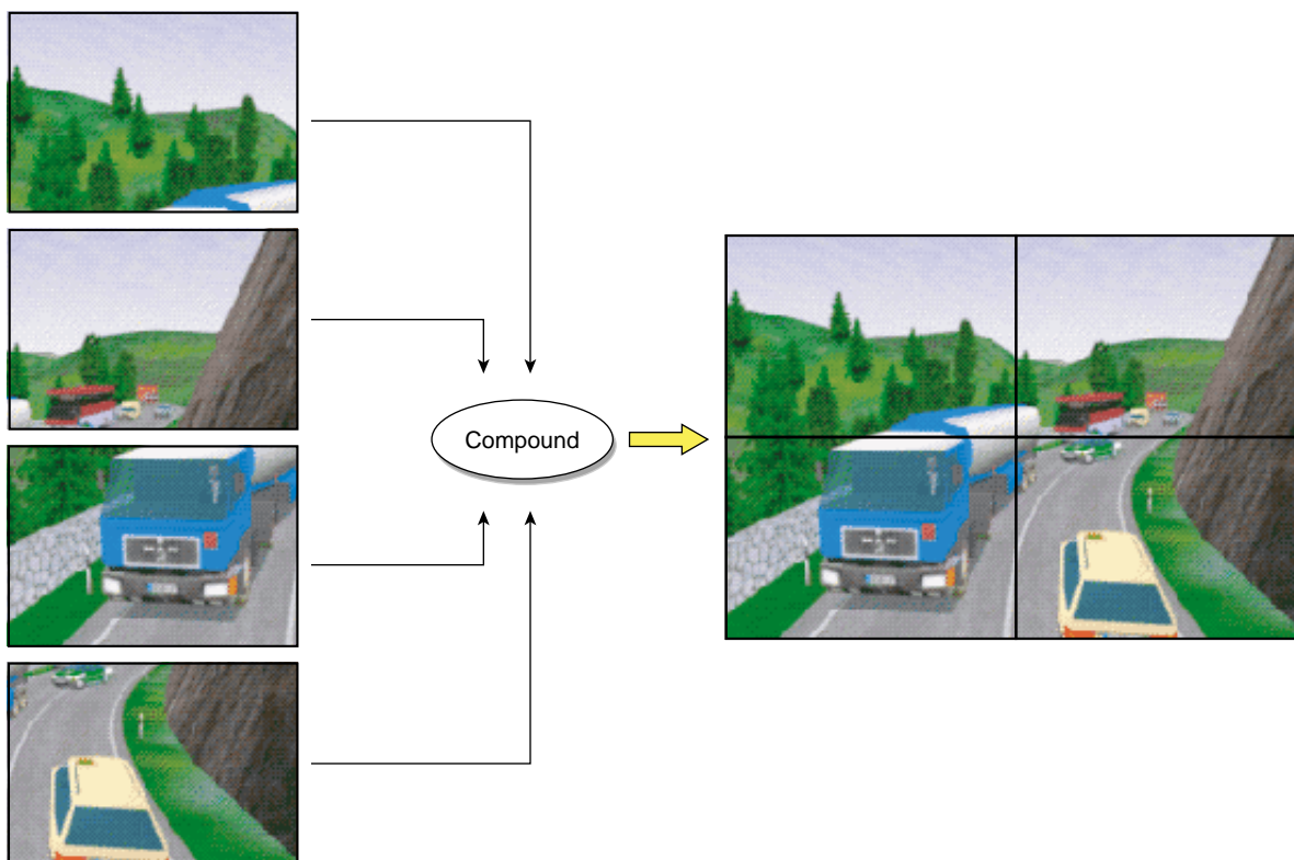
Figure 3-2 Screen Decomposition
