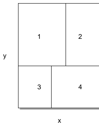
Figure 3-20 2D Tiling Scheme with Four Regions and Horizontal Tiles
