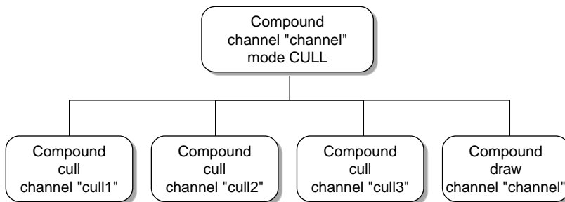
Figure 4-4 Multiple Cull Threads for a Single Channel
