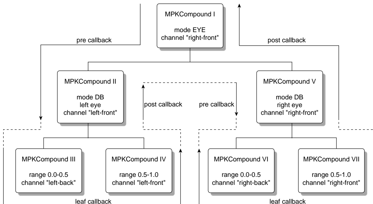
Figure 3-23 MPKCompound Traversal
